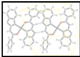
Fig. 2. Part of a [100] chain of molecules in the crystal of (I) with hydrogen bonds indicated by double-dashed lines.
